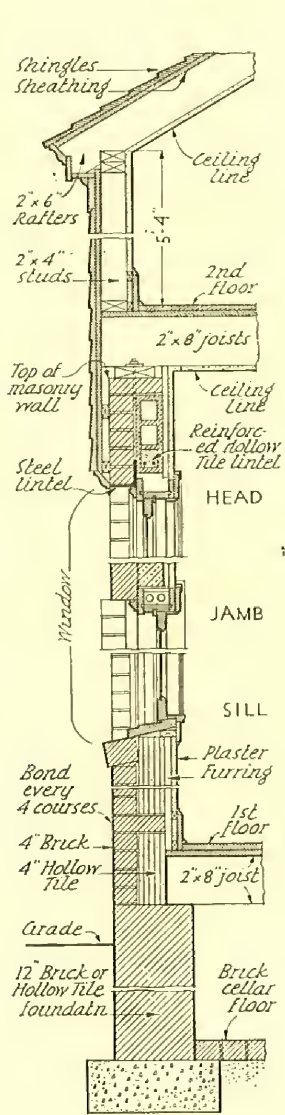
Wall Section
